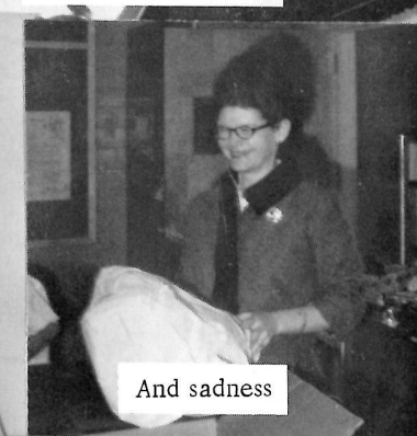
Assembly programs
